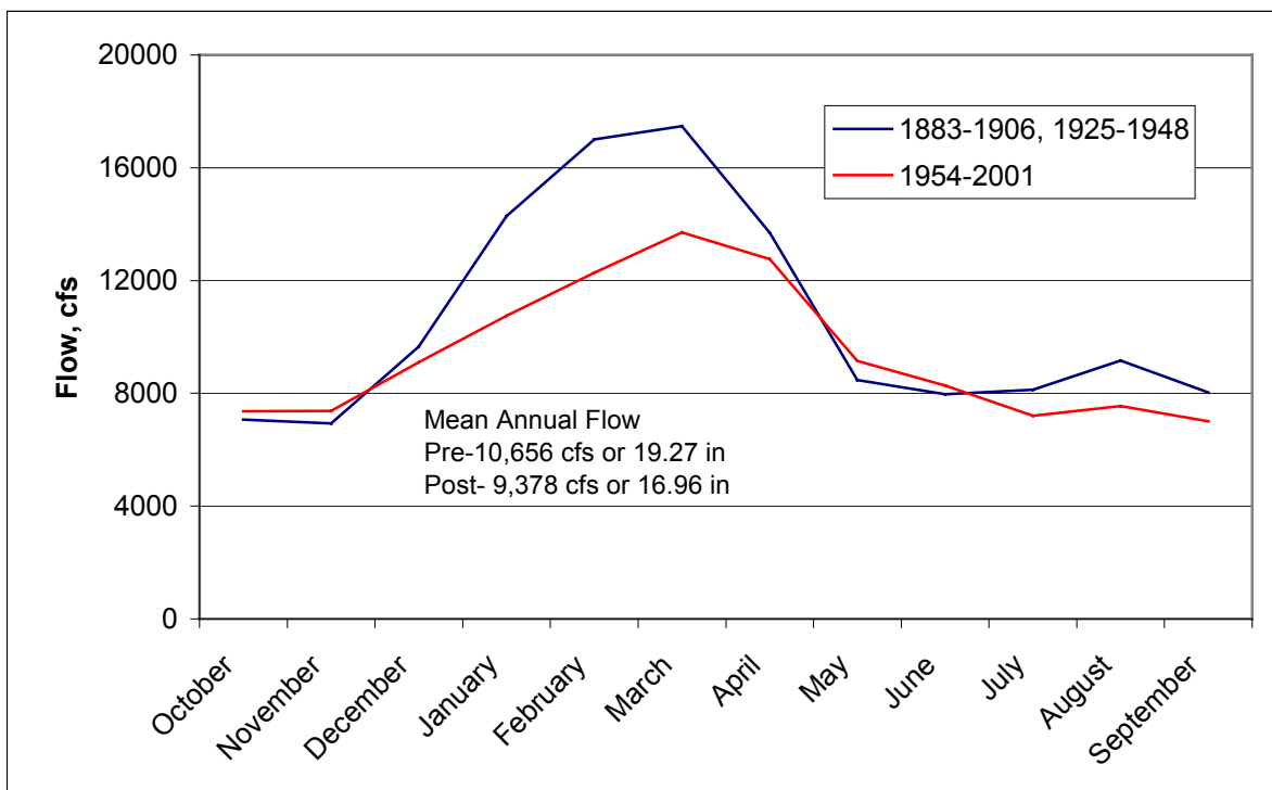
Figure 13b. Pre- and post-dam mean monthly flows for USGS gage #02198500 at Clyo.
